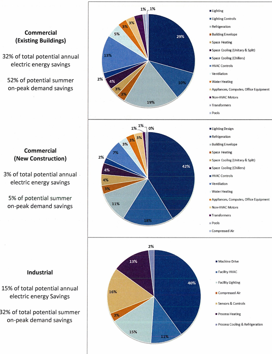
Figure 29. Maximum Achievable Commercial and Industrial Electric Savings Potential by End Use
