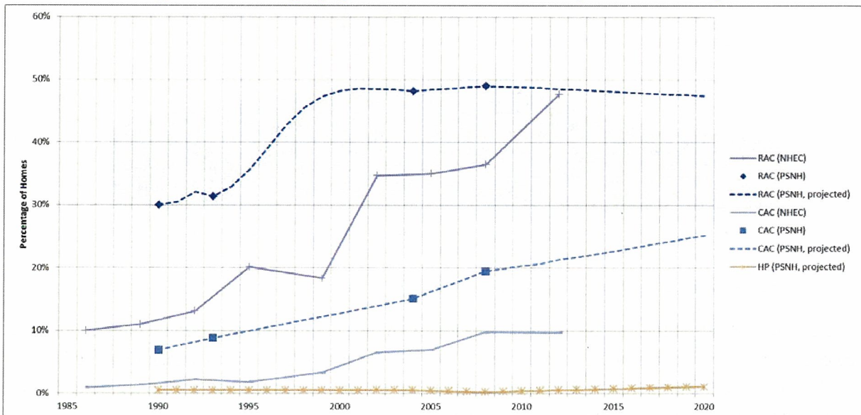
Figure E-2. Cooling Equipment in Residential Sector (PSNH and NHEC)
