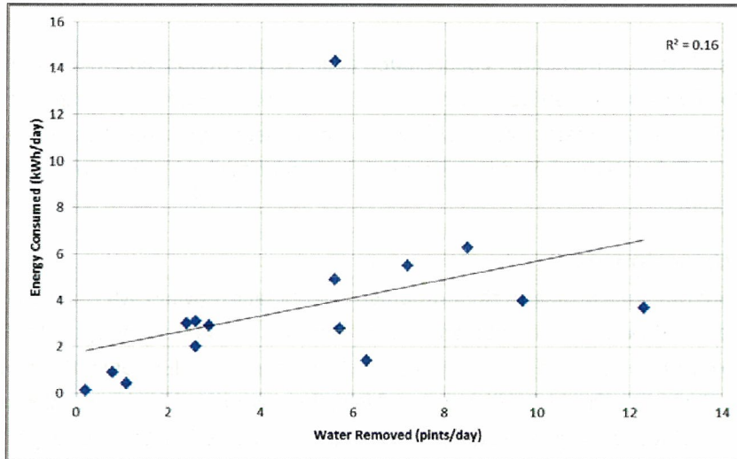
Figure 27. Daily Electricity Use of a Dehumidifier
