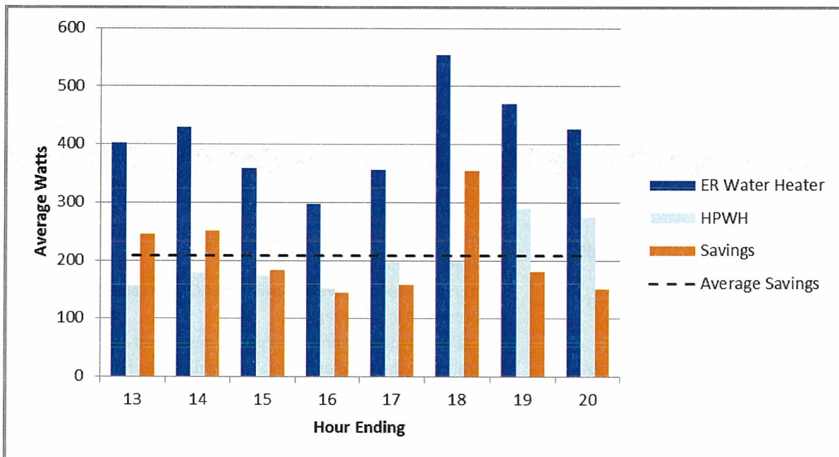
Figure 30. Peak Savings for a Heat Pump Water Heater
